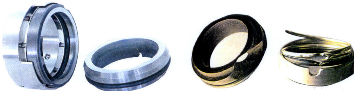
Damaged mech. seal
